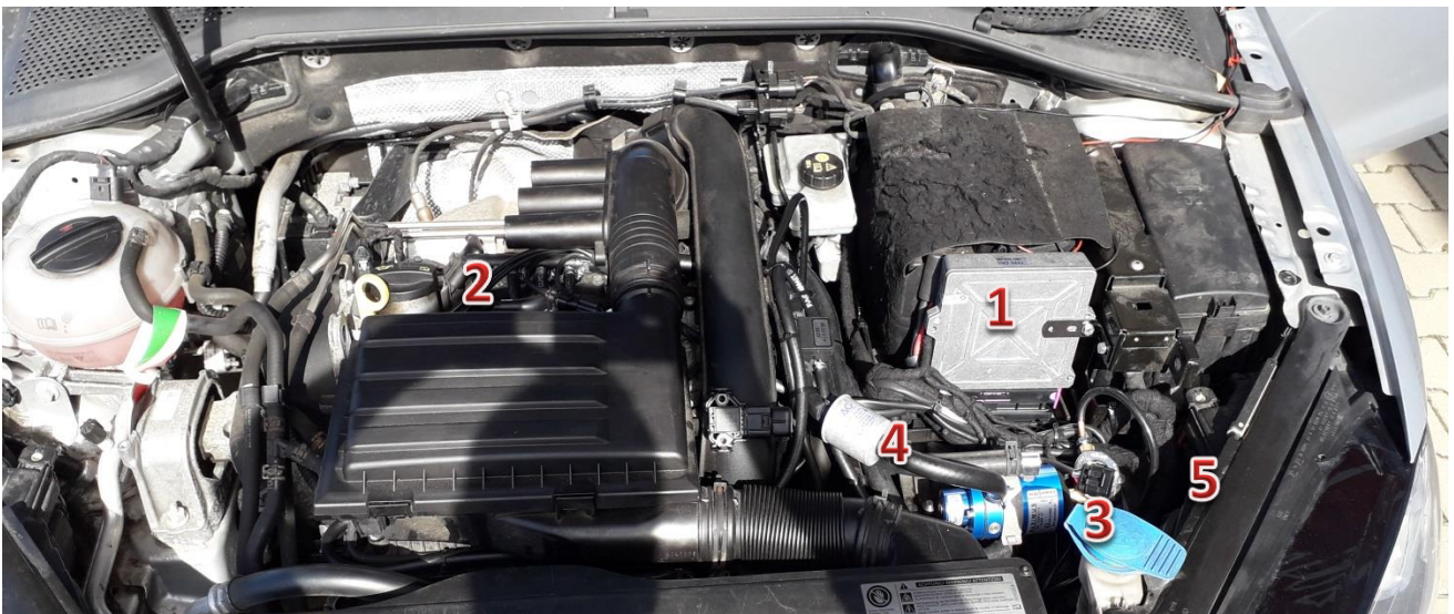
1-sterownik/ECU Zenit Direct, 2-wtryskiwacze gazu/gas injectors, 3-reduktor/reducer, 4-filtr fazy lotnej/gas phase filter, 5-elektrozawór z filtrem fazy ciekłej/electrovalve with liquid gas phase filter
